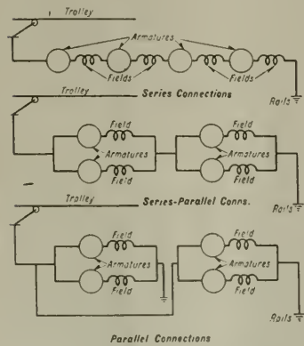
FIG. 1—MOTOR COMBINATIONS
